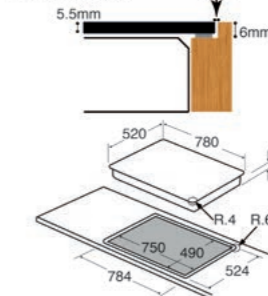
Flush installation
