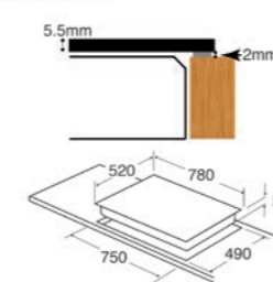
Inset installation
